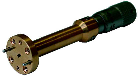
Tunable waveguide short
