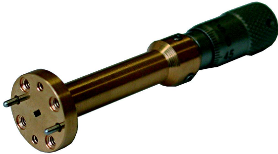
Sliding Matched Load
